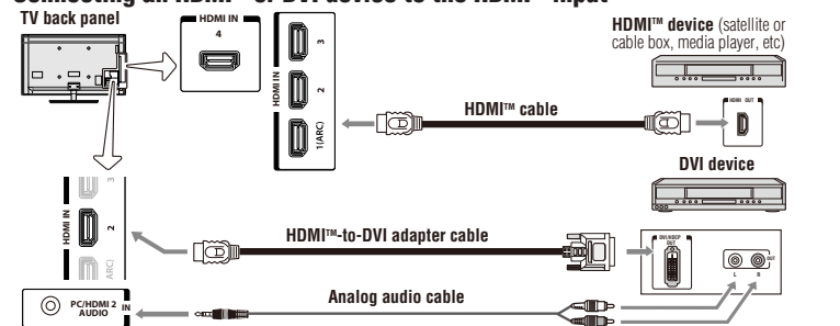
(Sample Illustration) HDMI™ and DVI connections
