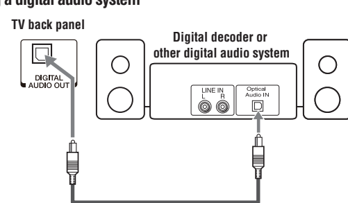
(Sample Illustration) Connecting a digital audio system
