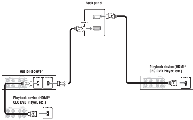
(Sample Illustration) 58/65L5400U—HDMI® CEC compatible audio receiver and playback device connections
