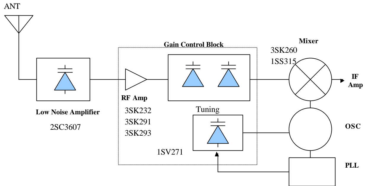
Fig. 1. Toshiba RF ICs in a Digital TV Tuner
