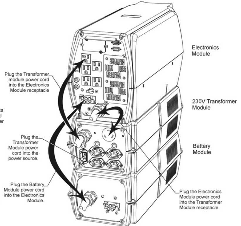
Figure 3: 230V Transformer Module Configuration
