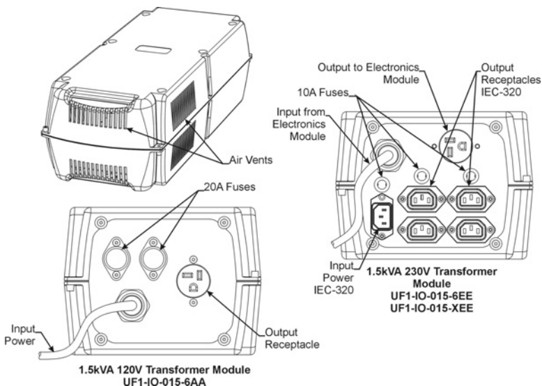
Figure 1 Module Layout
