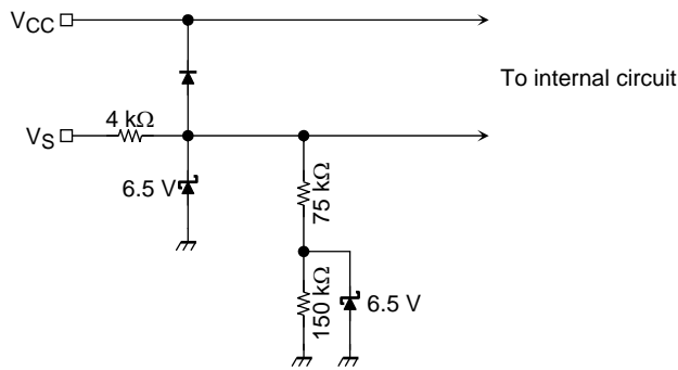
Internal circuit diagram of VS pin
