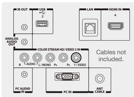
Rear Panel Connector Diagram
