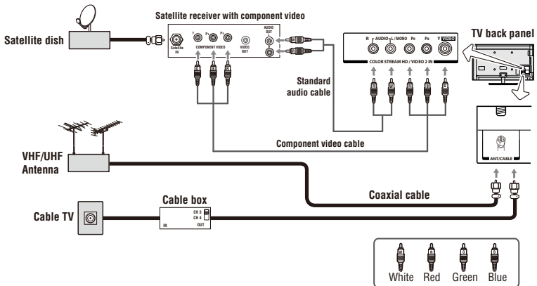
(Sample Illustration) L9300U Series—Connecting to an antenna, satellite receiver, and/or cable TV box
