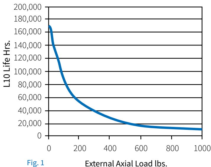
L10 Life Vs. External Axial Load
