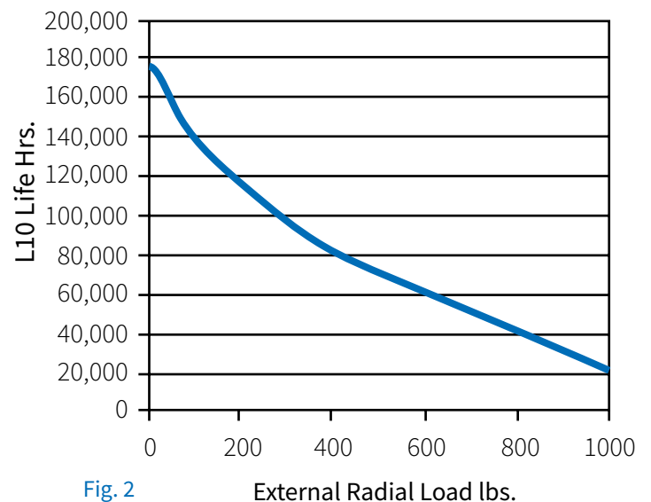
L10 Life Vs. External Radial Load
