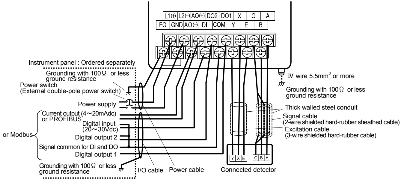
Figure 6. Separate type LF470/LF622 flowmeters wiring Diagram
