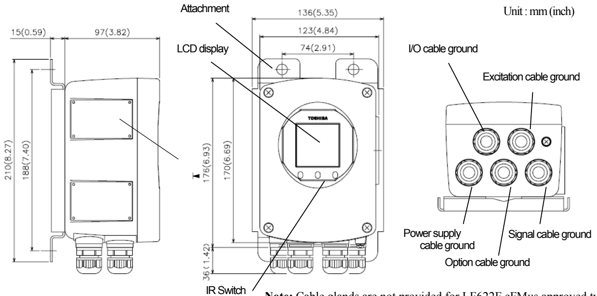
Figure3. LF470 Dimensions
