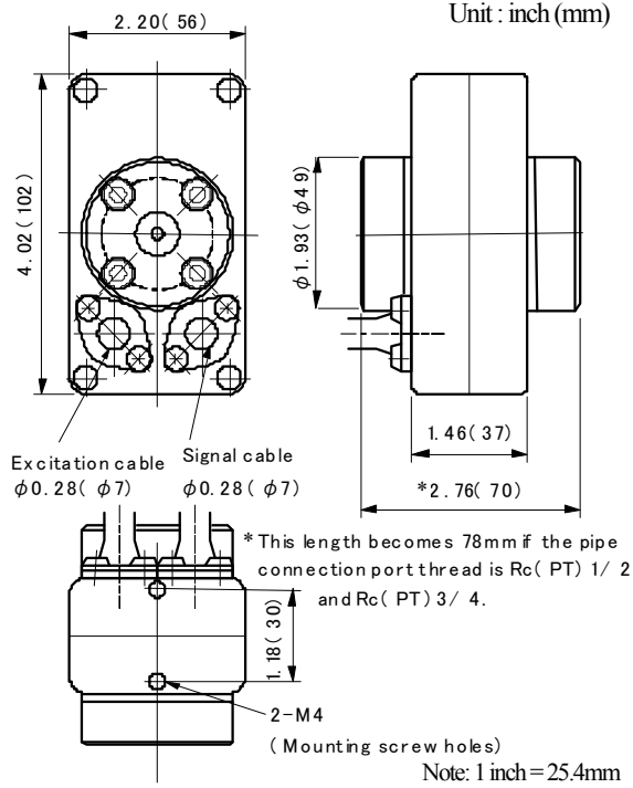
Figure3. LF470 Dimensions
